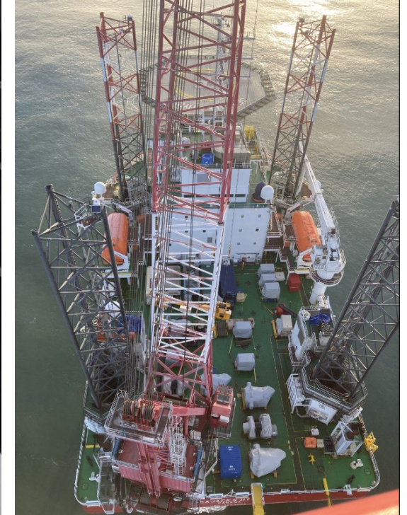
Undertaking turbine maintenance using jack up vessels
